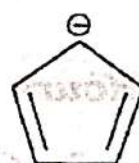
Cyclopentadienyl anion
