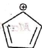
Cyclopentadienyl cation
