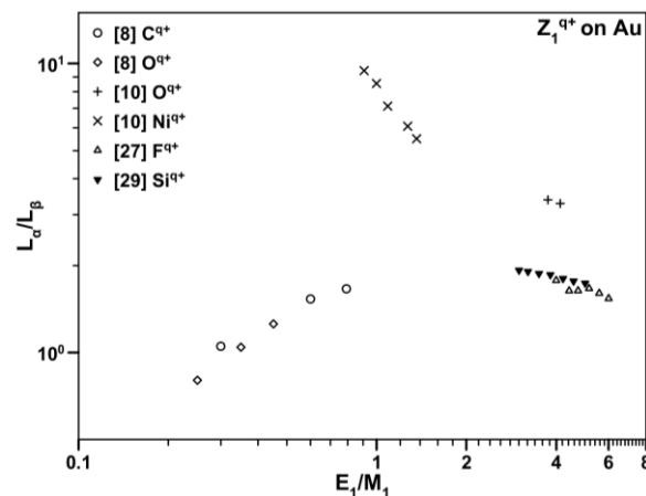
Figure 7. L_\alpha/L_\beta ratio obtained for various authors (Table 1) for collision of different ions with Au.
