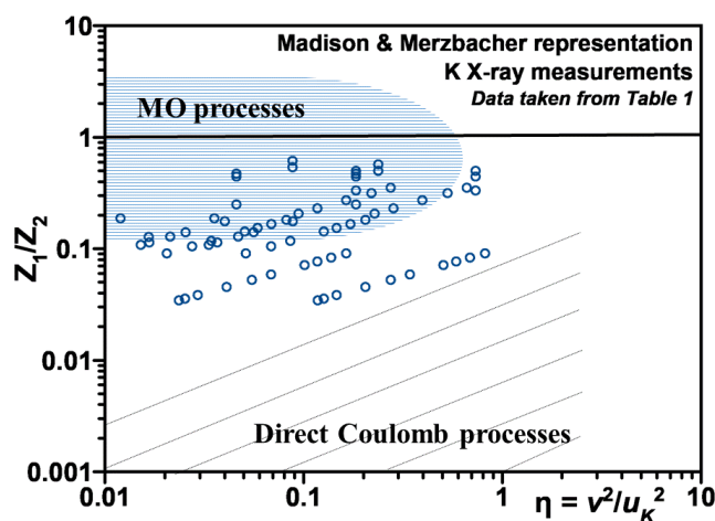
Figure 3. Madison and Merzbacher map equivalent for systems investigated using K-shell X-rays from Table 1 [5-7, 17, 19, 21, 22, 25].
