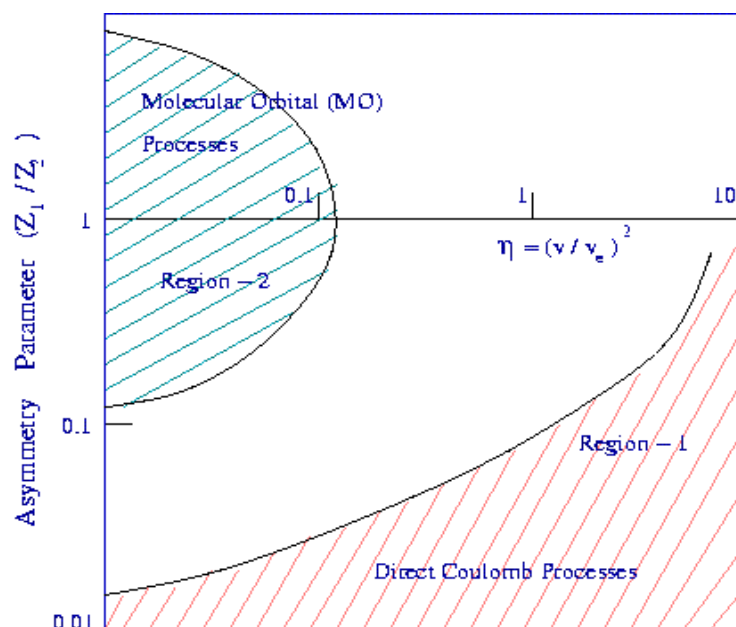
Figure 1. Regions of validity of various approximations in general semiclassical theory of inner-shell electrons by Madison and Merzbacher showing Z_1/Z_2 as a function of the adiabaticity parameter, \eta . Here, v_e is the orbital velocity of the target inner-shell electrons, which is denoted by u_s in the text. The domains for direct Coulomb and molecular orbital (MO) processes are distinctly defined here [2]. The region \eta < 1 is the quasi-adiabatic region.
