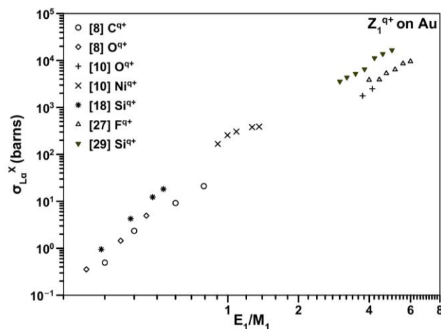
Figure 6. L_{\alpha} line production cross sections ( \sigma ; X denotes X-ray) reported by various authors (Table 1) for collision of different ions with Au ( q = charge state of the ions).
