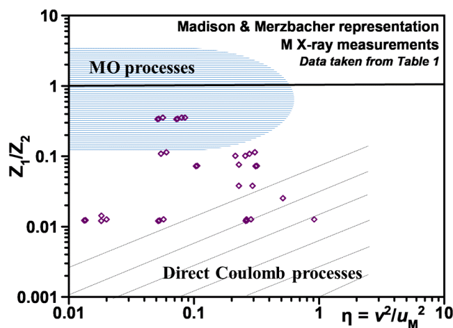
Figure 5. Madison and Merzbacher map equivalent for systems investigated using M-shell X-rays from Table 1 [14, 16, 23, 24, 28, 30, 32, 33].
