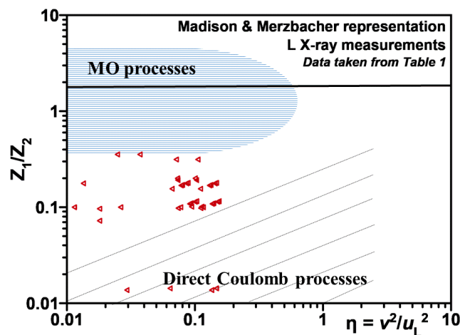
Figure 4. Madison and Merzbacher map equivalent for systems investigated using L-shell X-rays from Table 1 [8-14, 15, 18, 20, 21, 29, 31].
