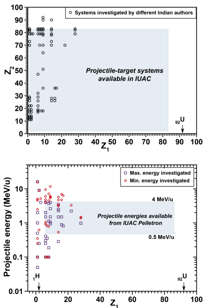
Figure 2. Summary of systems from Table 1 according to atomic numbers. Here the blue rectangles indicate those systems that are available at IUAC. The shaded regions show those systems and energies that are available and can be investigated easily in IUAC, India.
